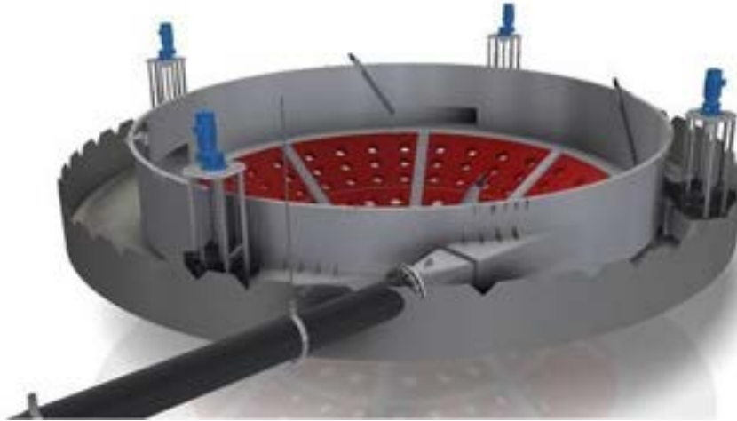
Figure 6: HydroForce – Froth management system
