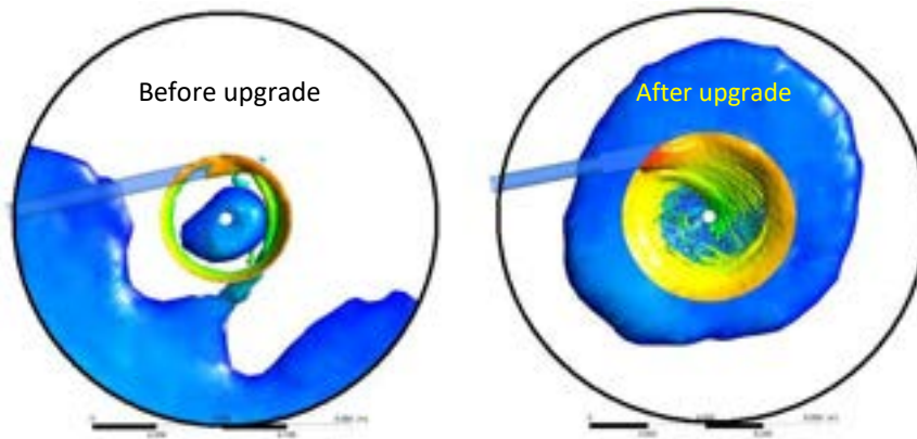
Figure 2: CFD models of even distribution into the thickener – Before and after Vector® upgrade
