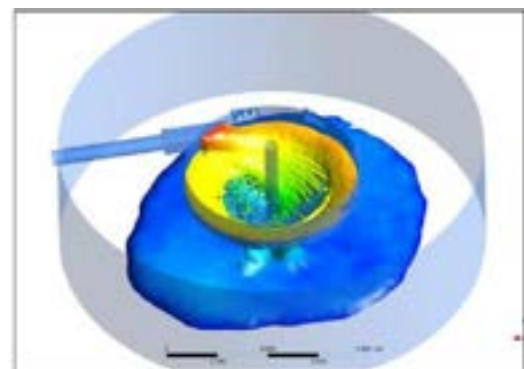
Figure 1: Velocity through Vectors® showing the even distribution into the thickener
