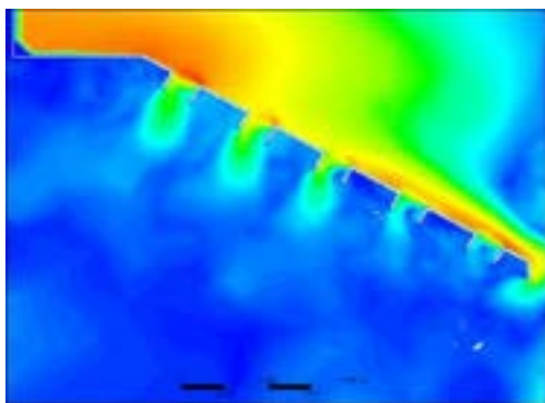
Figure 1: Velocity through Vectors® showing the even distribution into the thickener
